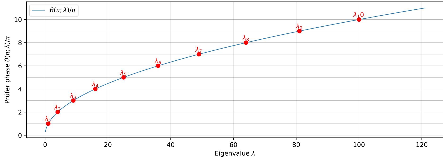
Prüfer phase sweep on clustered grid (n=100, 70%/30%) for 10 eigenvalues
